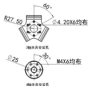
Fixture size
