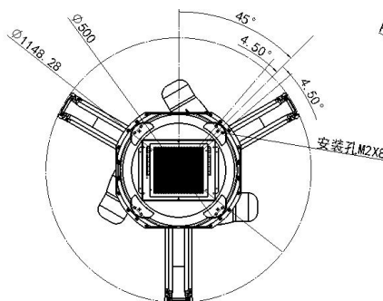
Installation size
