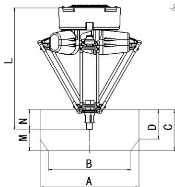
Working reach
