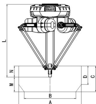
Working reach
