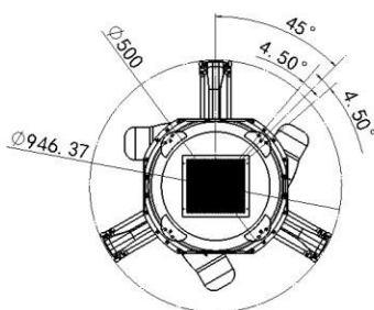
Installation size
