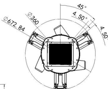
Installation size
