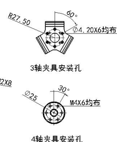
Fixture size
