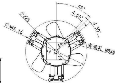
Installation size
