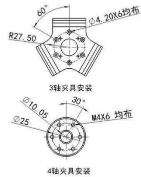
Fixture size
