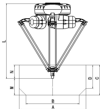
Working reach
